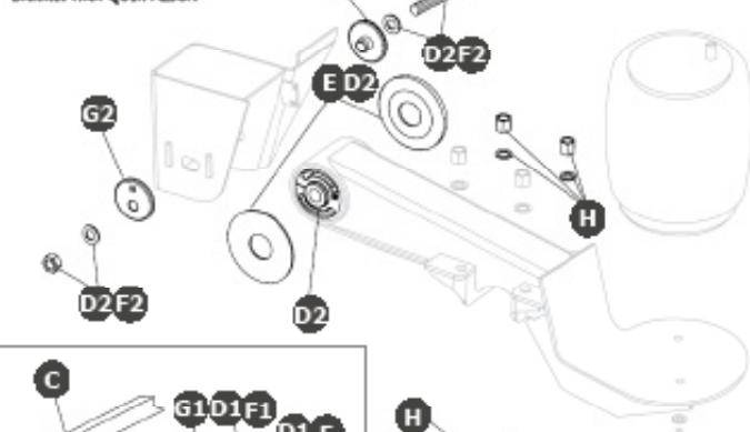
Winged, Weld-On Frame Bracket with QUICK-ALIGN
