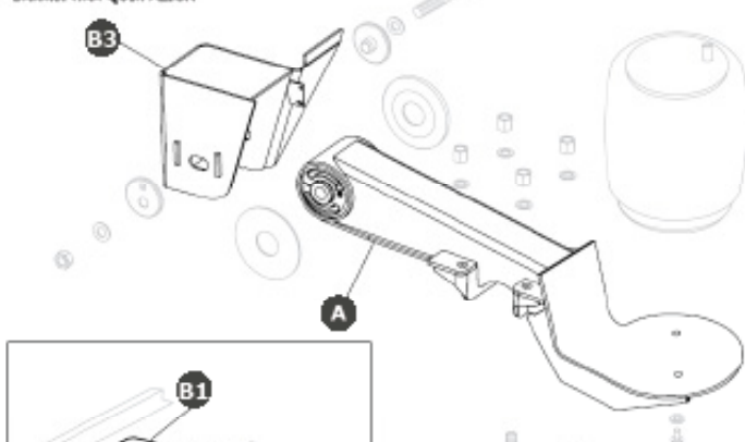
Winged, Weld-On Frame Bracket with QUICK-ALIGN
