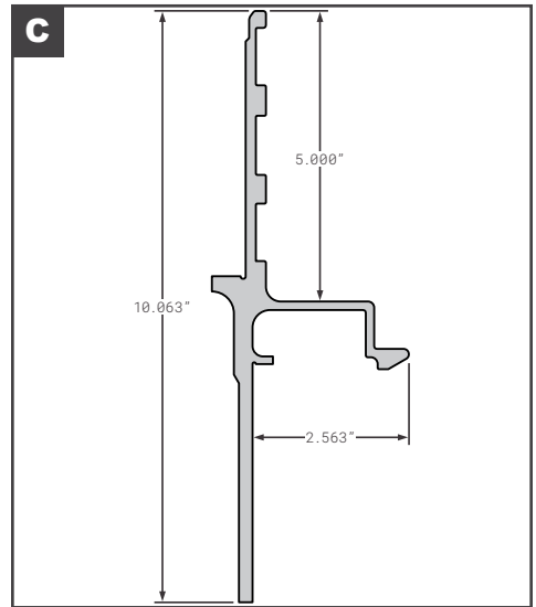
Lift Pads
