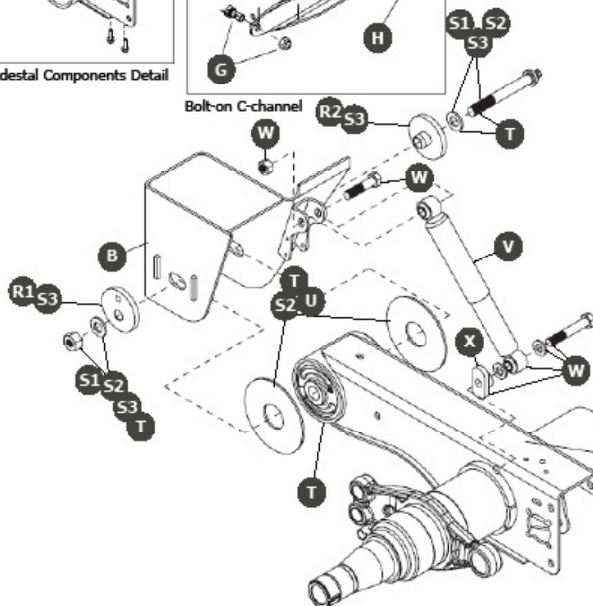
LDA Axle, cast pedestal
