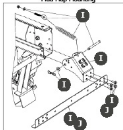
Mud Flap Mounting
