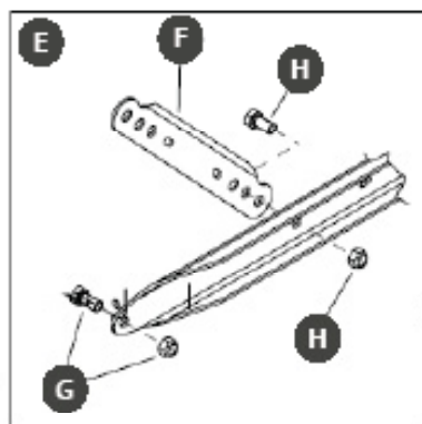
Bolt-on C-channel
