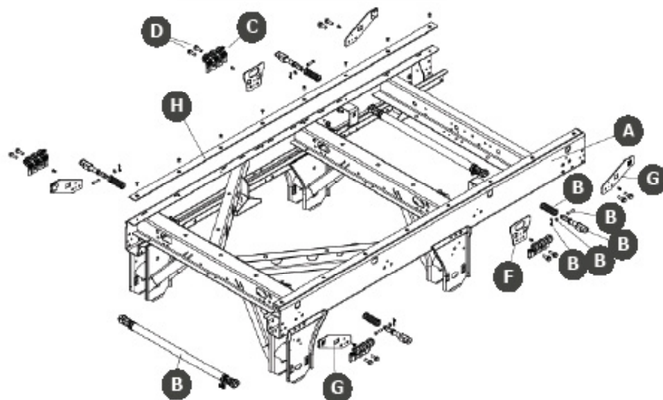
Mud Flap Mounting
