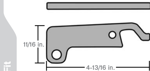
Safety Latch TWL-LA001
