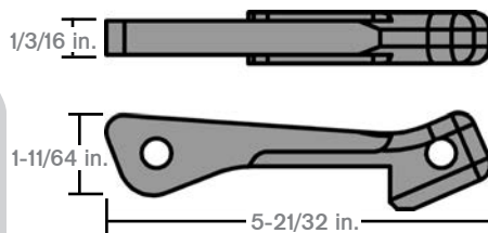
Lock Latch TWL-LA006
