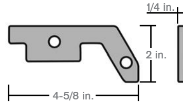
Safety Latch TWL-LA010
